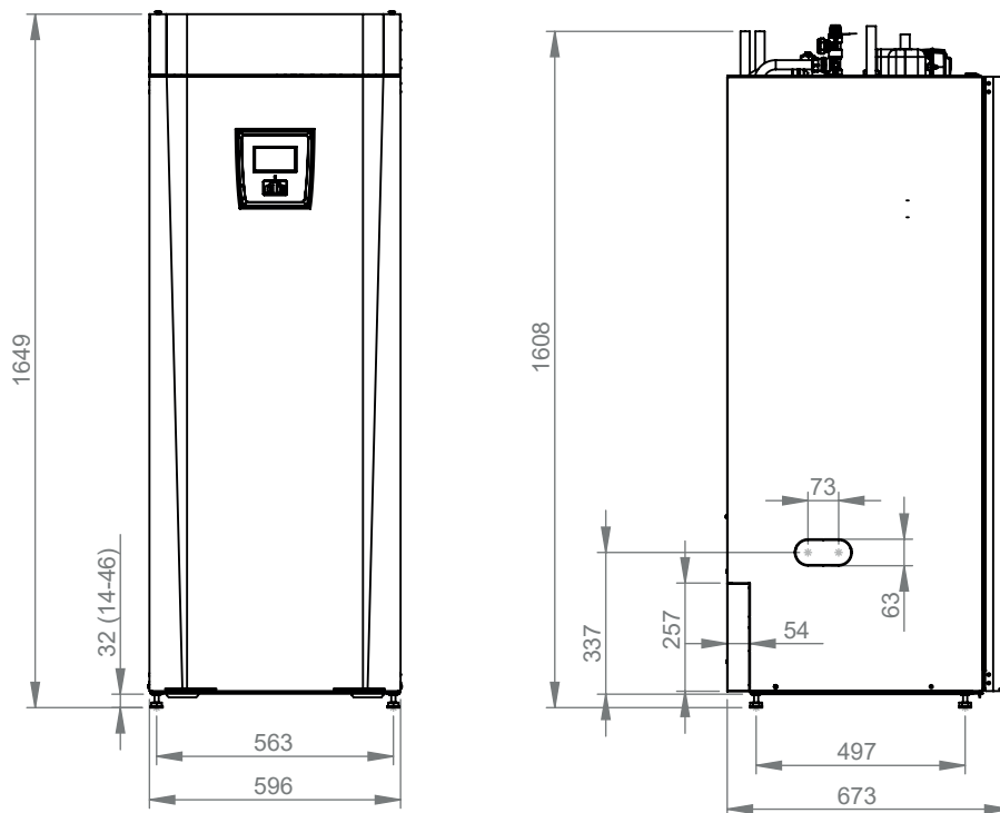
Visok model - CTC EcoZenit i255H
