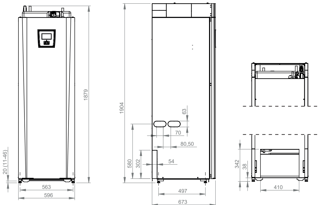
Visok model - CTC EcoZenit i255H
